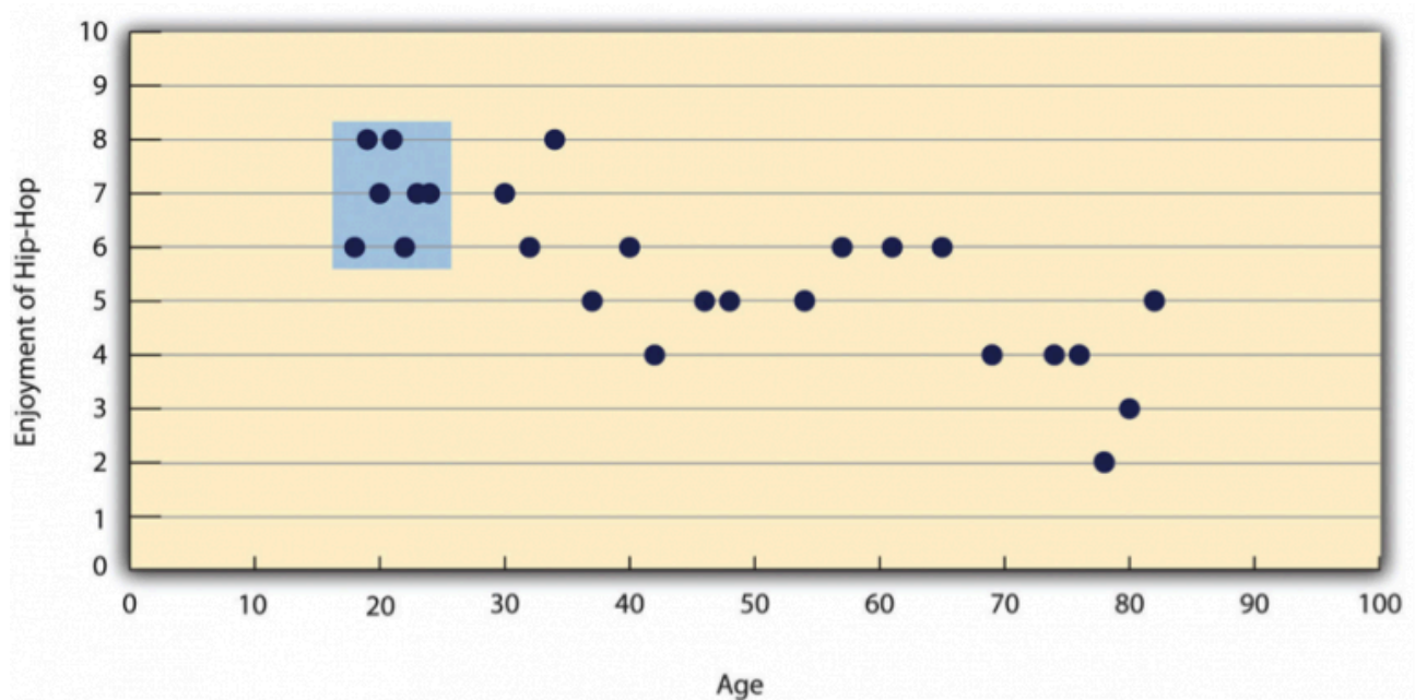
Figure 10.4.6. Hypothetical data showing how a strong overall correlation can appear to be weak when one variable has a restricted range. The overall correlation here is -.77 , but the correlation for the 18- to 24-year-olds (in the blue box) is 0, by R. S. Jhangiani et al. in Research Methods in Psychology 4e is used under a CC BY-NC-SA licence
