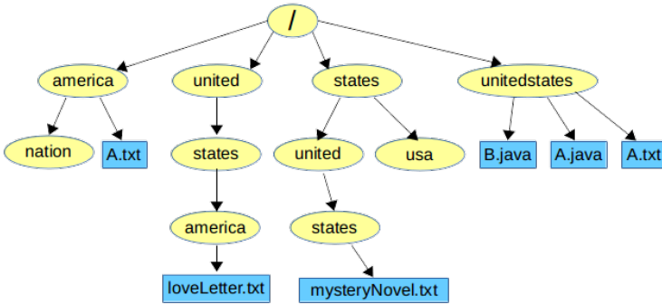
Figure 1.1: The Linux filesystem, in pictorial form.
