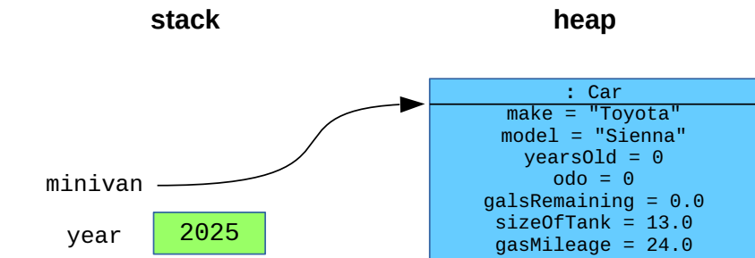
Figure 4.1: The stack and the heap.
