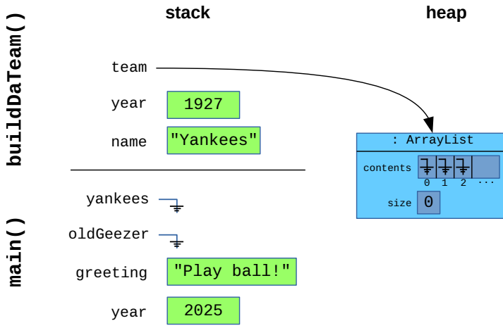
Figure 4.7: Memory contents after calling the function and executing the first three lines of buildDaTeam() .
