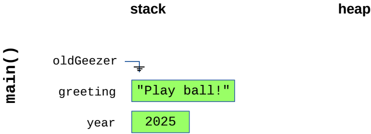
Figure 4.6: Memory contents after executing the first three lines of main() .
