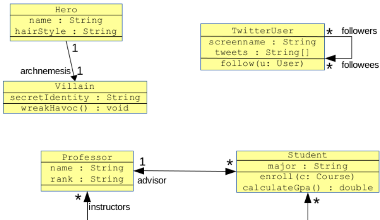
Figure 6.10: Association annotations indicating roles.
