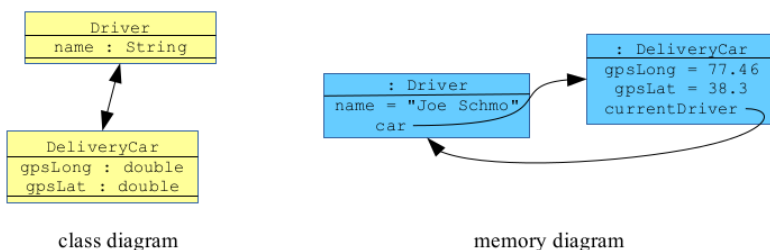
Figure 6.5: A bidirectional “has-a,” depicted on a class diagram (left) and a memory diagram.
