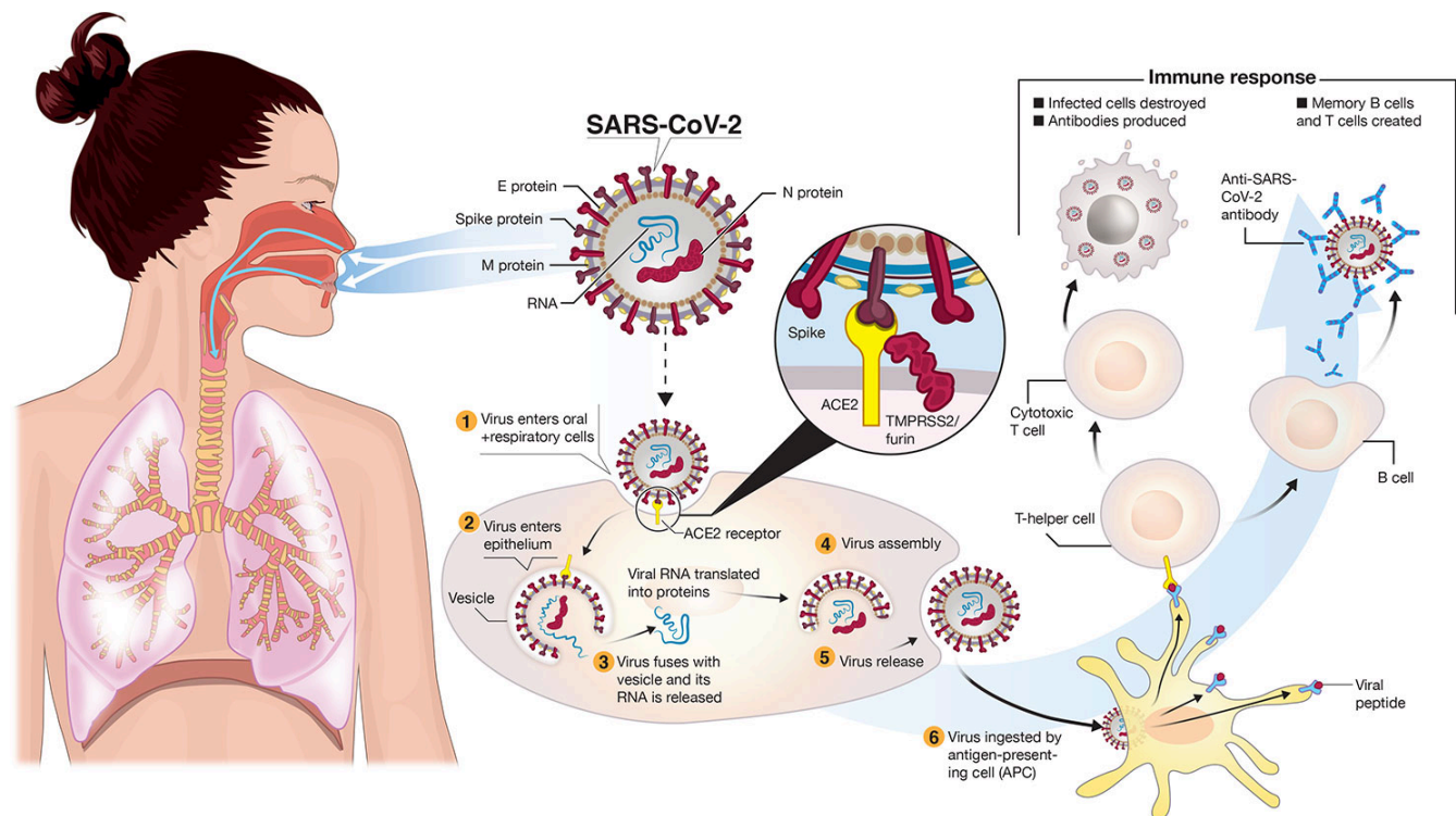
Figure 13.2.1 Transmission and Life-Cycle of SARS-CoV-2 Causing COVID-19. SARS-CoV-2 is transmitted via respiratory droplets of infected cases to oral and respiratory mucosal cells. The virus, possessing a single-stranded RNA genome wrapped in nucleocapsid (N) protein and three major surface proteins: membrane (M), envelope (E) and Spike, replicates and passes to the lower airways potentially leading to severe pneumonia. The gateway to host cell entry (magnified view) is via Spike-converting enzyme 2 (ACE2) interaction with cleavage of Spike in the prefusion state by proteases TMPRSS-2/furin. A simplified depiction of the life cycle of the virus is shown along with potential immune responses elicited. [ Long description ]
