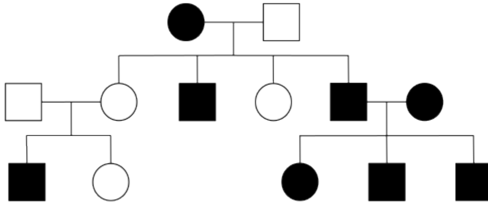
Figure 4.3.4 A Pedigree Consistent with X-Linked Recessive Inheritance [Long description]
