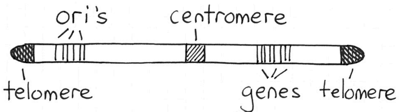
Figure 12.1.1 Parts of a Typical Human Nuclear Chromosome (Not to Scale). The ori 's and genes are distributed everywhere along the chromosome, except for the telomeres and centromere. [ Long description ]
