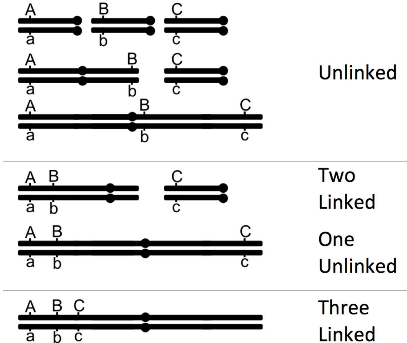
Figure 11.3.5 Examples of How Three Genes can be Associated with Each Other, Based on Whether All Three are Unlinked, All Three are Linked, or Two are Linked and One Unlinked [ Long description ]
