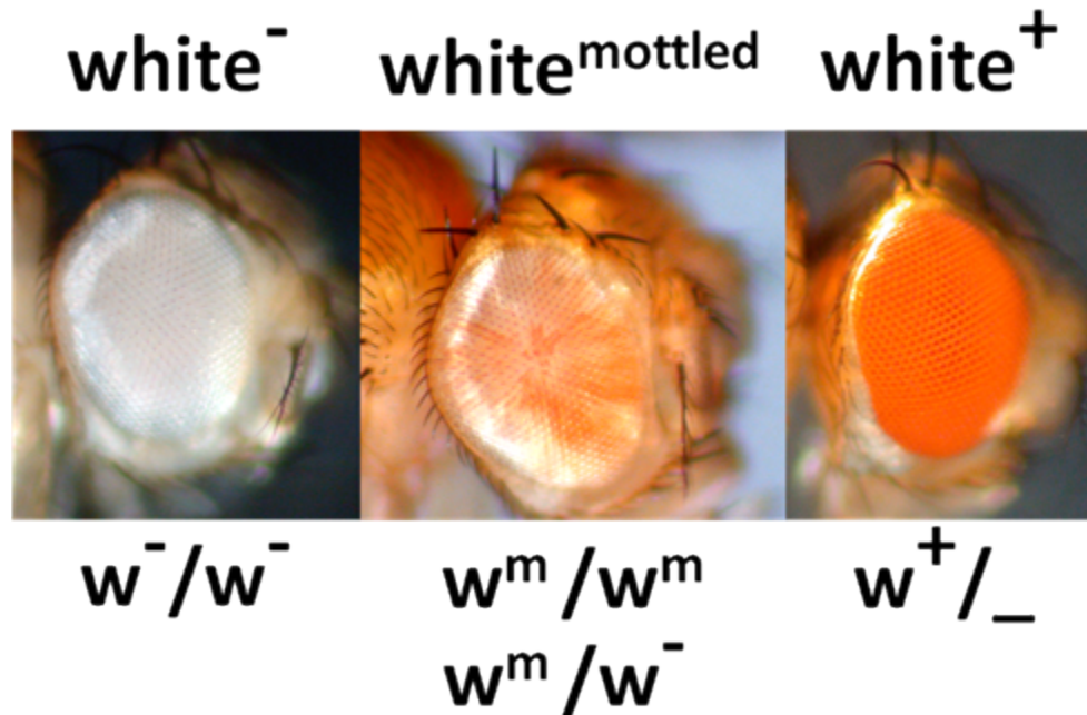
Figure 8.3.9 Mutation in the White Gene Impacts the Pigmentation in Drosophila Eyes. Note. White mottled is recessive to w^+ and dominant to w^- [ Long description ]
