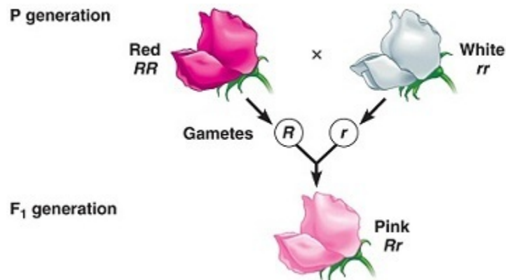
Figure 6.5.3 Incomplete Dominance (Blended Phenotype Produced) [ Long description ]
