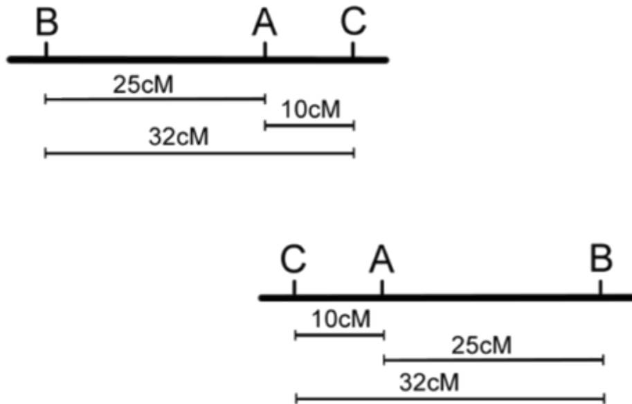
Figure 11.3.4 Two Possible Maps Based on the Data in Table 11.3.2 (Without Correction for Double Crossovers) [ Long description ]
