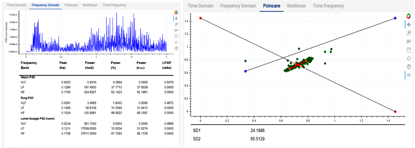
Fig.7. Frequency Domain and Poincare Analysis
