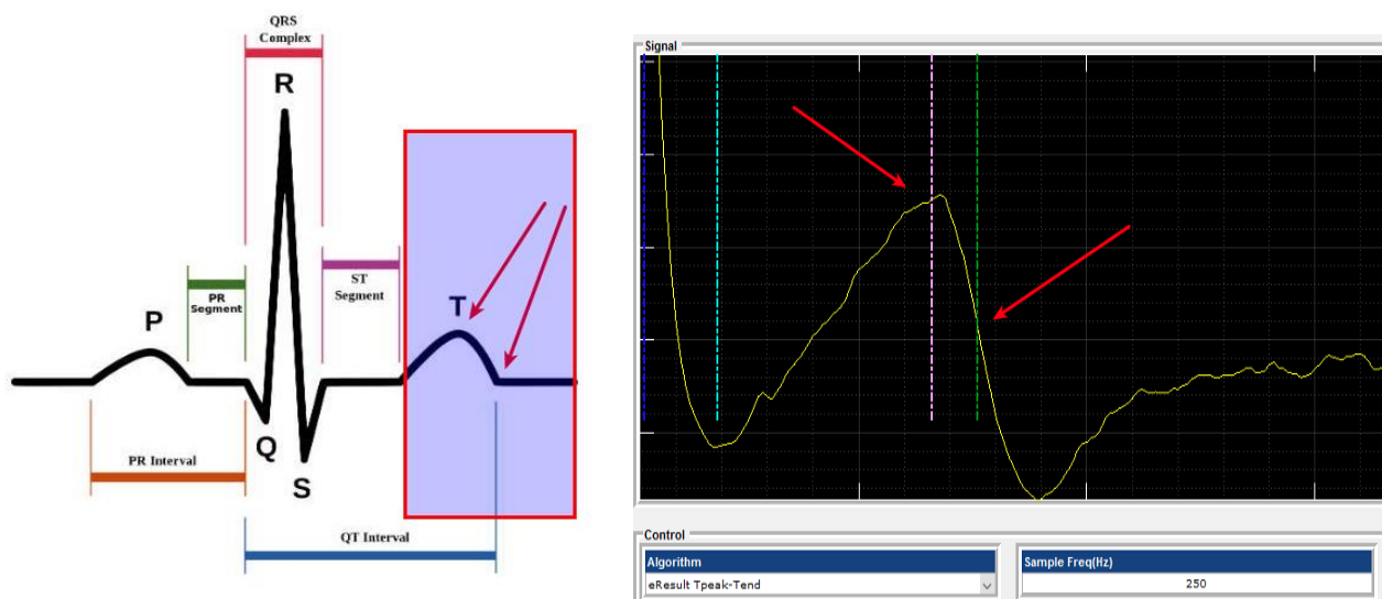
Fig.3. TpTe determination
