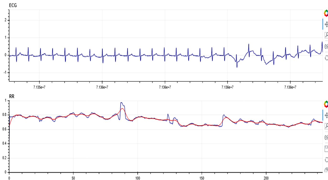
Fig.5. Arrhythmic beats and artefacts
