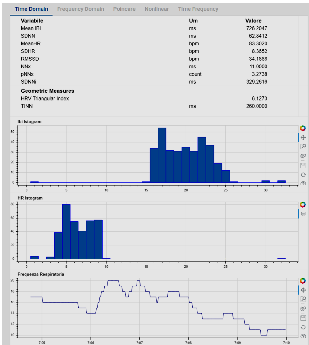
Fig.6. Time Domain Analysis
