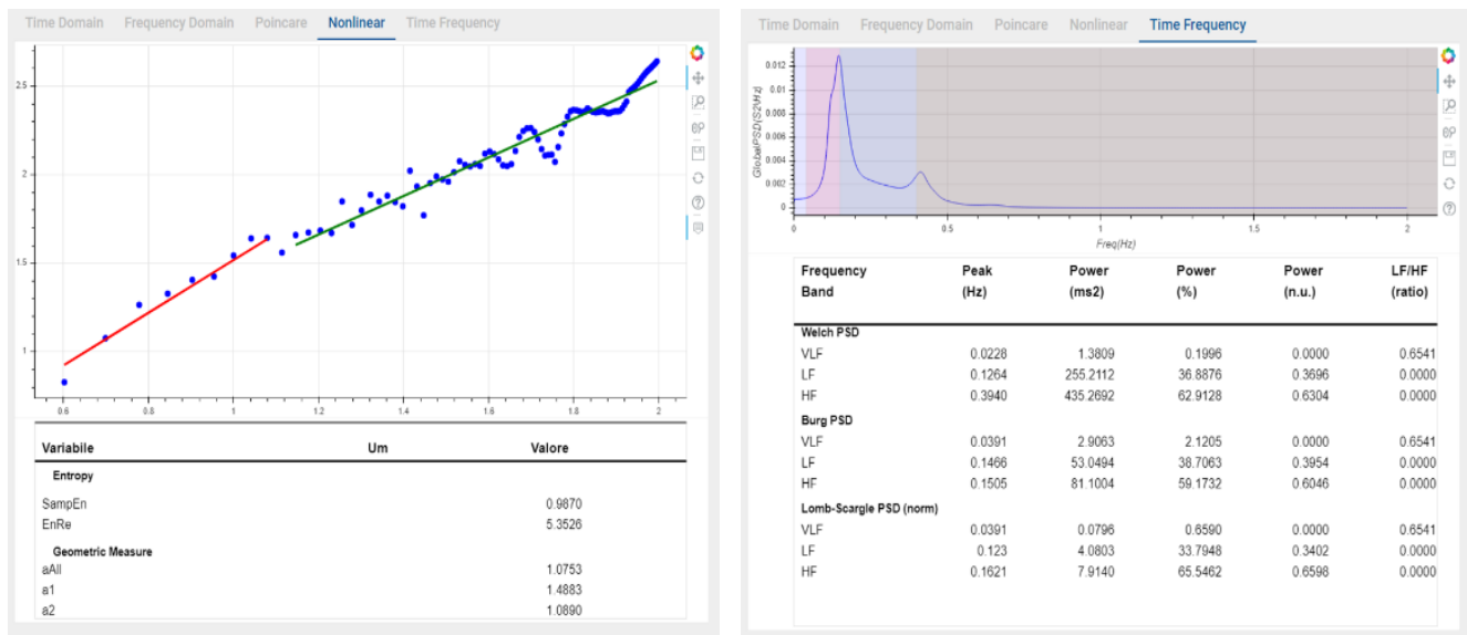
Fig.8. Nonlinear and Time Frequency Analysis
