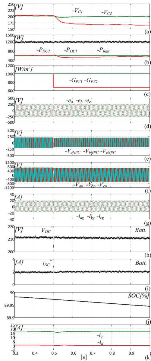
Figure 11. Six-level MMC- G_{PV2} drop from 1000 W/m 2 to 700 W/m 2 . (a) String voltages V_{c1} and V_{c2} . (b) ES 1 , ES 2 , and energy storage system (ESS) output power. (c) G_{PV1} and G_{PV2} . (d) Grid voltage. (e) NPC output voltage. (f) Primary voltage. (g) Grid current. (h) Battery voltage. (i) Current. (j) State of charge (SOC). (k) Output d,q axes currents.
