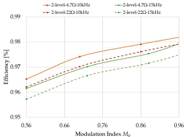
Figure 13. Efficiency of the three-phase 2L inverter as a function of modulation depth M_0 with I_C = 15 \text{ m} , V_{BUS} = 400 \text{ V} , I_x = 30 \text{ A} .
