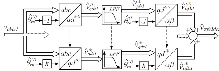
Figure 4. Block diagram of the multiharmonic SRF filtering (MSF) algorithm.
