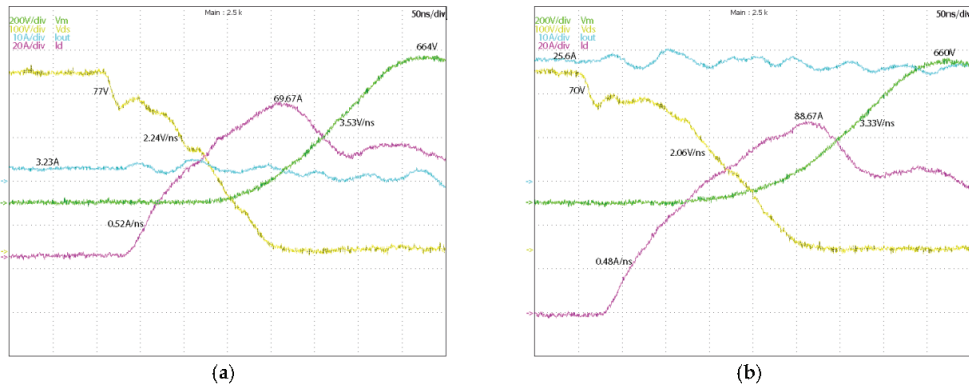
Figure 11. Turn-on of S_{A,t} located in the three-phase S2L inverter with R_G = 4.7\ \Omega , C_{S_{A,t}} = 9.4\ \mu\text{F} dead-time DT = 1\ \mu\text{s} , switching frequency f_{sw} = 10\ \text{kHz} and l_C = 15\ \text{m} : (a) phase current of 3.23 A, (b) phase current of 25.6 A. Line-to-line voltage V_m at the motor side (green track), drain-source voltage V_{DS} of the S_{A,t} (yellow track), drain current of S_{A,t} (magenta track) and phase current I_A (ciano track).
