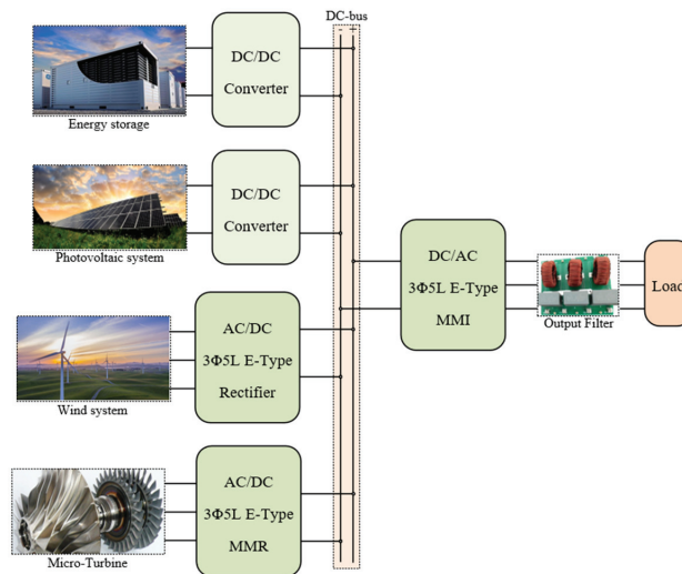
Figure 1. Structure of stand-alone microgrid with the integrated renewable energy source.
