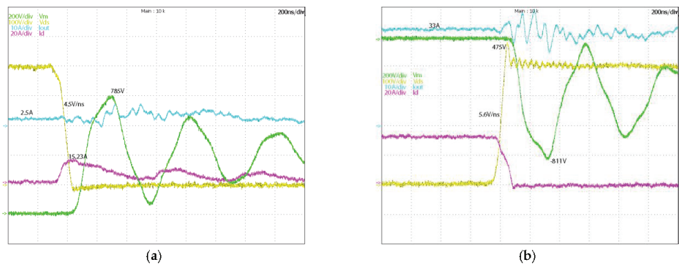
Figure 10. Commutation of S_{A,t} located in the three-phase 2L inverter with R_G = 22\Omega , dead-time DT = 1\mu s , switching frequency f_{sw} = 10\text{ kHz} and l_C = 15\text{ m} : (a) turn-off, (b) turn-on. Line-to-line voltage V_m at the motor side (green track), drain-source voltage V_{DS} of the S_{A,t} (yellow track), drain current of S_{A,t} (magenta track) and phase current I_A (ciano track).
