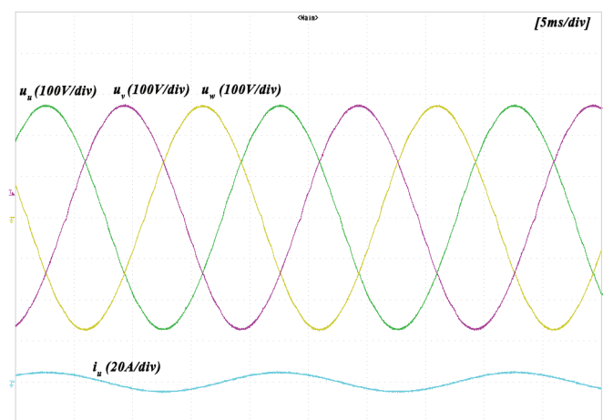
Figure 20. Phase-to-neutral voltages u_u, u_v, u_w of the 3Φ5L E-Type MMI side under resistive load.
