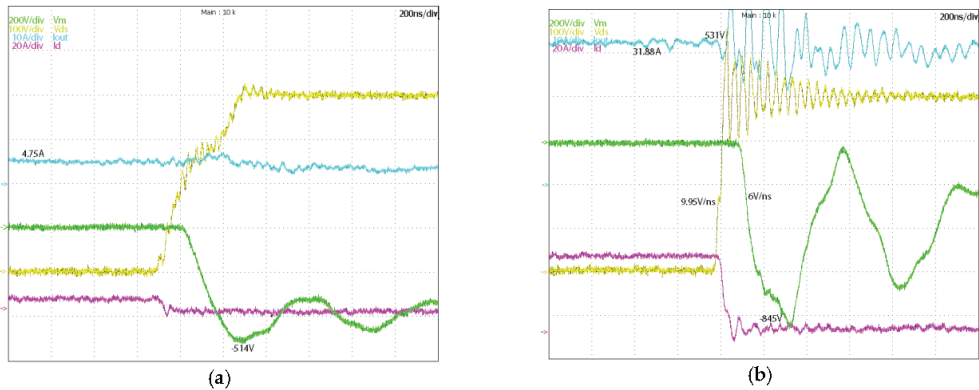
Figure 9. Turn-off of S_{A,t} located in the three-phase 2L inverter with R_G = 4.7\Omega , dead-time DT = 1\mu s , switching frequency f_{sw} = 10\text{ kHz} and l_C = 15\text{ m} : (a) phase current of 4.75\text{ A} , (b) phase current of 31.88\text{ A} . Line-to-line voltage V_m at the motor side (green track), drain-source voltage V_{DS} of the S_{A,t} (yellow track), drain current of S_{A,t} (magenta track) and phase current I_A (ciano track).
