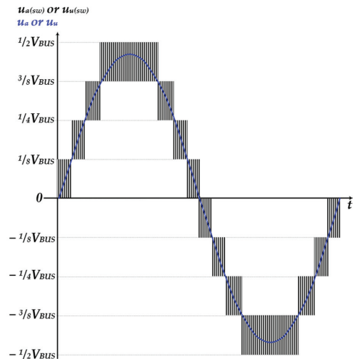
Figure 5. Line-to-line switching voltage u_{a(sw)} (or u_{u(sw)} ).
