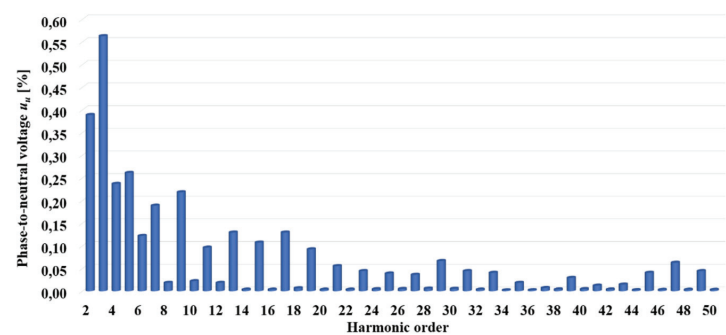
Figure 21. Harmonic spectrum of the phase-to-neutral voltage u_u .
