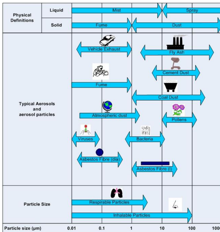
Figure 6.1 - Particle Sizes
