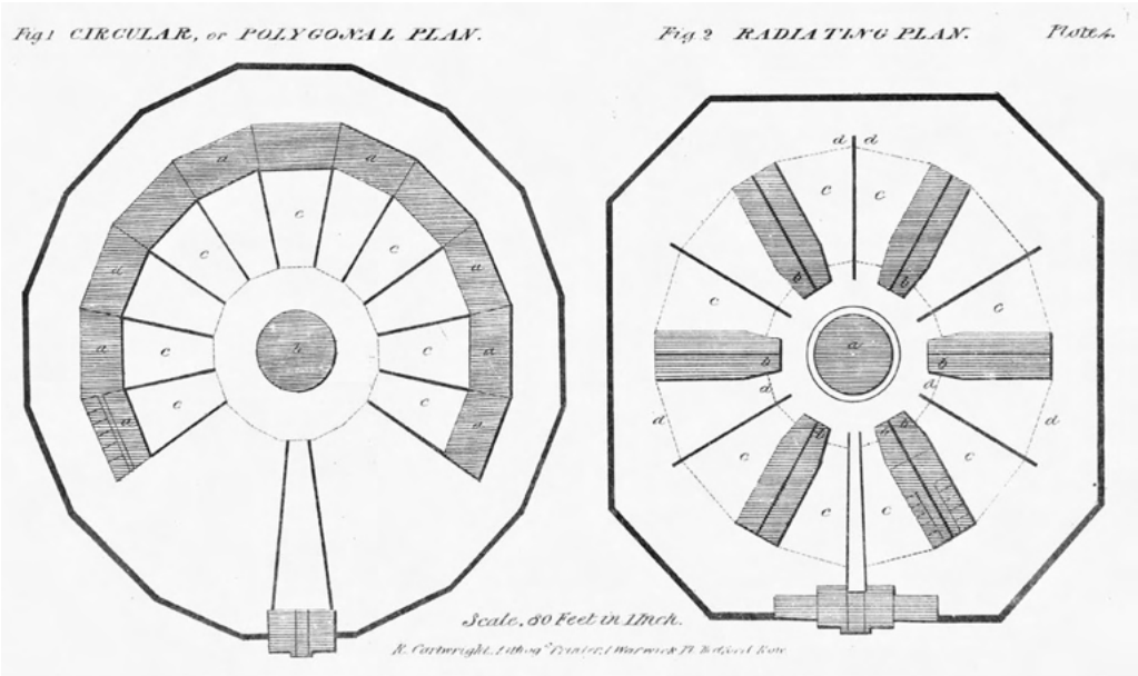
54 Contrasting forms: polygonal versus radial prison floor plans, 1828
