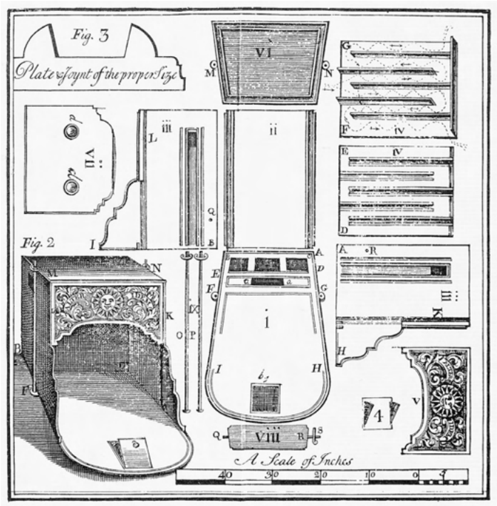
4 Assembly kit: construction drawings for Benjamin Franklin's Pennsylvania fireplace, 1744
