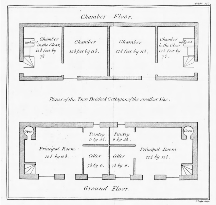
64-65 From landowners for land laborers: model plan for a semi-detached cottage by Nathaniel Kent, 1775
