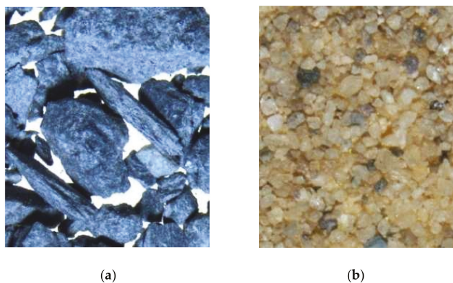
Figure 13. The difference in particle angularity between (a) shale (angular) and (b) sand (subrounded).
