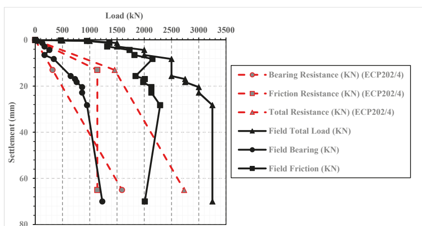
Figure 15. Comparison between field measurements of Alzey case history, and calculated values of pile settlement, friction, bearing, and total ultimate load using a settlement-based method [23].
