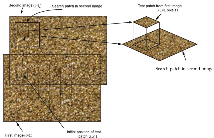
Figure 15. The principles of PIV technology.
