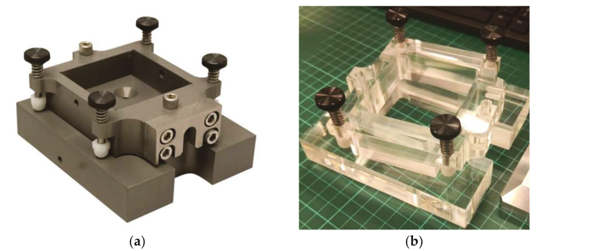
Figure 18. (a) A 60-mm (2.36 in) shear box (HMA-734MS) and (b) custom-made 60-mm (2.36 in) transparent shear box by the authors for preliminary interface shear study.
