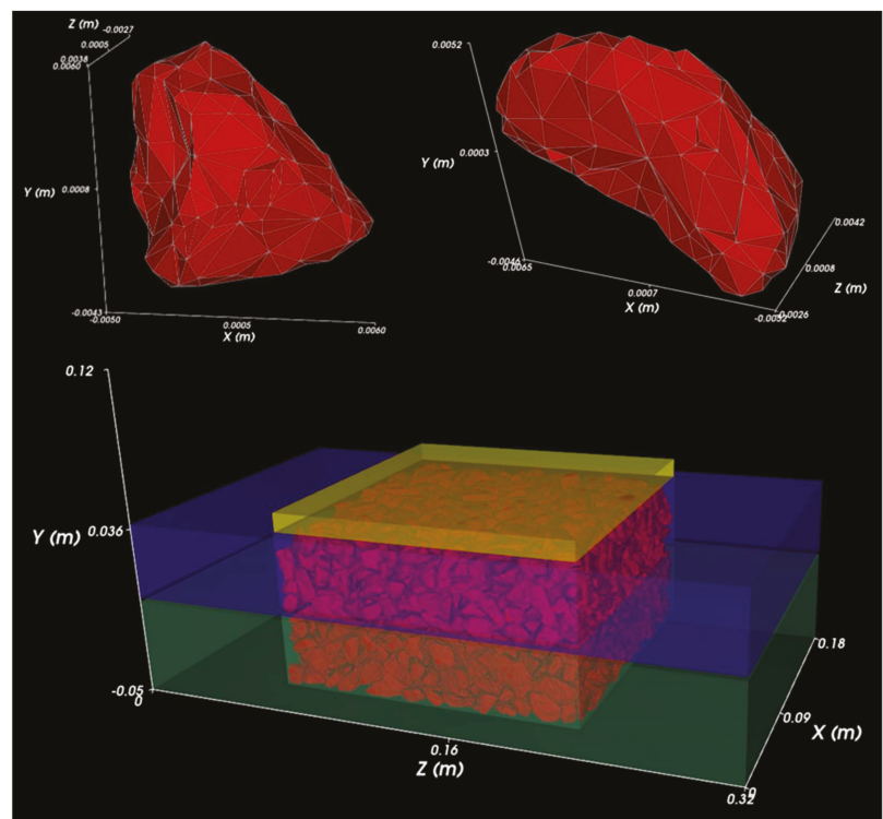
Figure 29. Realistic particle shapes are being used in DEM modeling as a revolutionary technique currently being developed by the authors.
