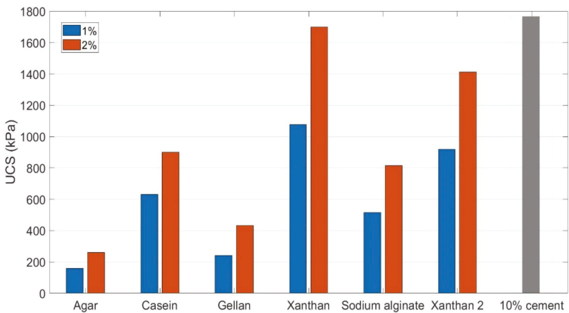
Figure 4. Biopolymer-treated sand [66,82,113,121,149–151].
