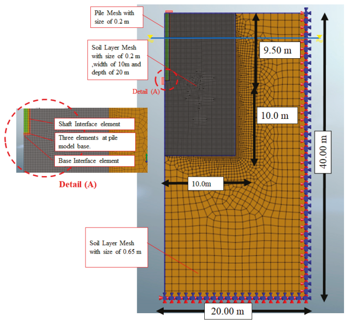
Figure 9. (2D) axisymmetric finite element model established based on the results of the sensitivity analysis performed (After [10]).
