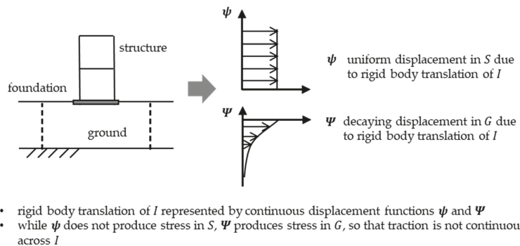
Figure 4. Displacement function induced by rigid body translation of interface.
