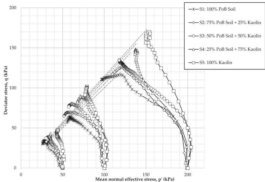
Figure 4. Effective stress paths for different confining pressures with varying silt contents (S1 represents 100% PoB soft soil; S2 represents 75% PoB soft soil + 25% kaolin soil; S3 represents 50% PoB soft soil + 50% kaolin soil, S4 represents 25% PoB soft soil + 75% kaolin soil; and S5 represents 100% kaolin soil; while 50,100, and 200 refer to the confining pressure.).
