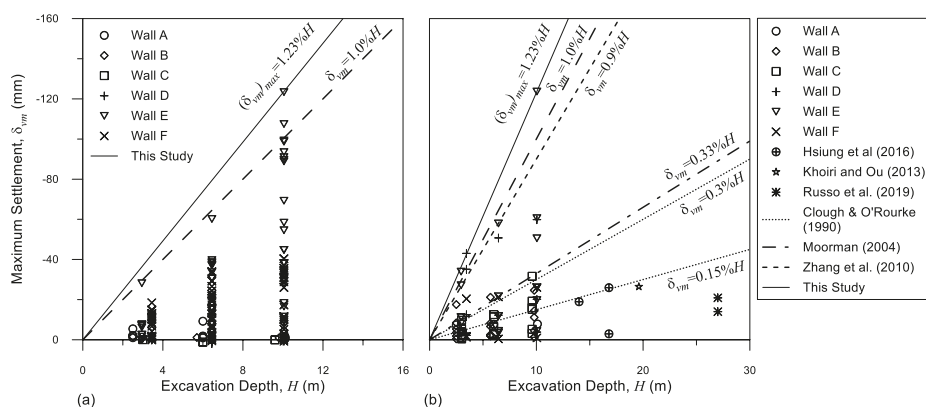
Figure 9. Relationship between maximum settlement and excavation depth for all the excavation stages for (a) building; and (b) ground.
