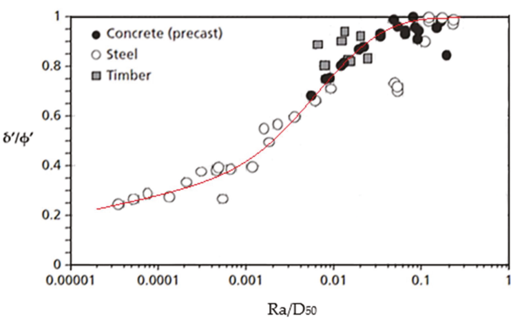
Figure 7. Interface friction angle for various construction materials.
