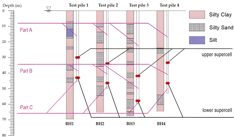
Figure 3. Subsurface conditions along test piles.
