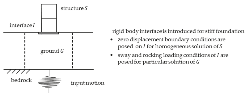
Figure 1. Schematic view of structure and ground.
