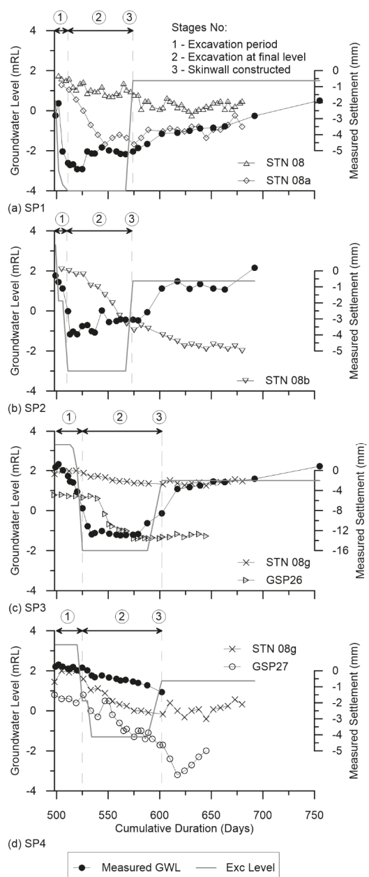
Figure 10. Measured groundwater and settlement profiles for (a) SP1; (b) SP2; (c) SP3; and (d) SP4.
