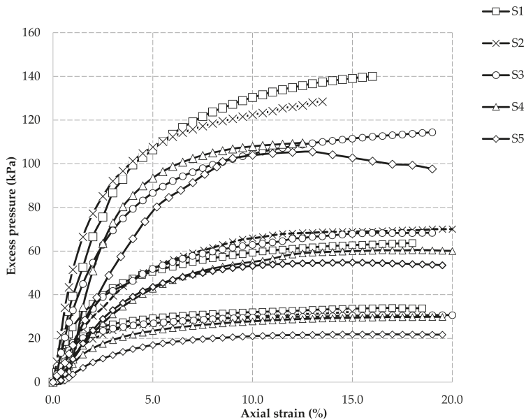
Figure 5. Excess pore pressure versus axial strain with different confining pressures for different silt contents. (S1 represents 100% PoB soft soil; S2 represents 75% PoB soft soil + 25% kaolin soil; S3 represents 50% PoB soft soil + 50% kaolin soil, S4 represents 25% PoB soft soil + 75% kaolin soil; and S5 represents 100% kaolin soil; while 50, 100, and 200 refer to the confining pressure.).
