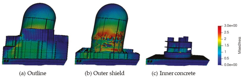
Figure 9. Deformation and the distribution of stress.
