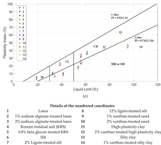
Figure 10. Variation of Atterberg limits by adding biopolymer, (a) liquid limit, (b) plasticity index, (c) plasticity chart [102,111,120,123,130,138,141,161].
